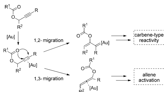
Scheme 1. Gold vinyl carbenoid and gold allenic intermediates.
