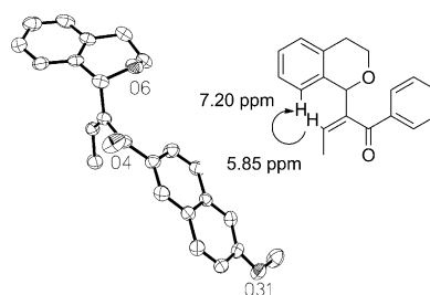
Figure 1. Left: Solid-state molecular structure of ( Z )- 3d (thermal ellipsoids at 50% probability); right: NOE observed in ( Z )- 3a .
